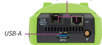
Main Ethernet Test Ports (RJ-45 & SFP)
